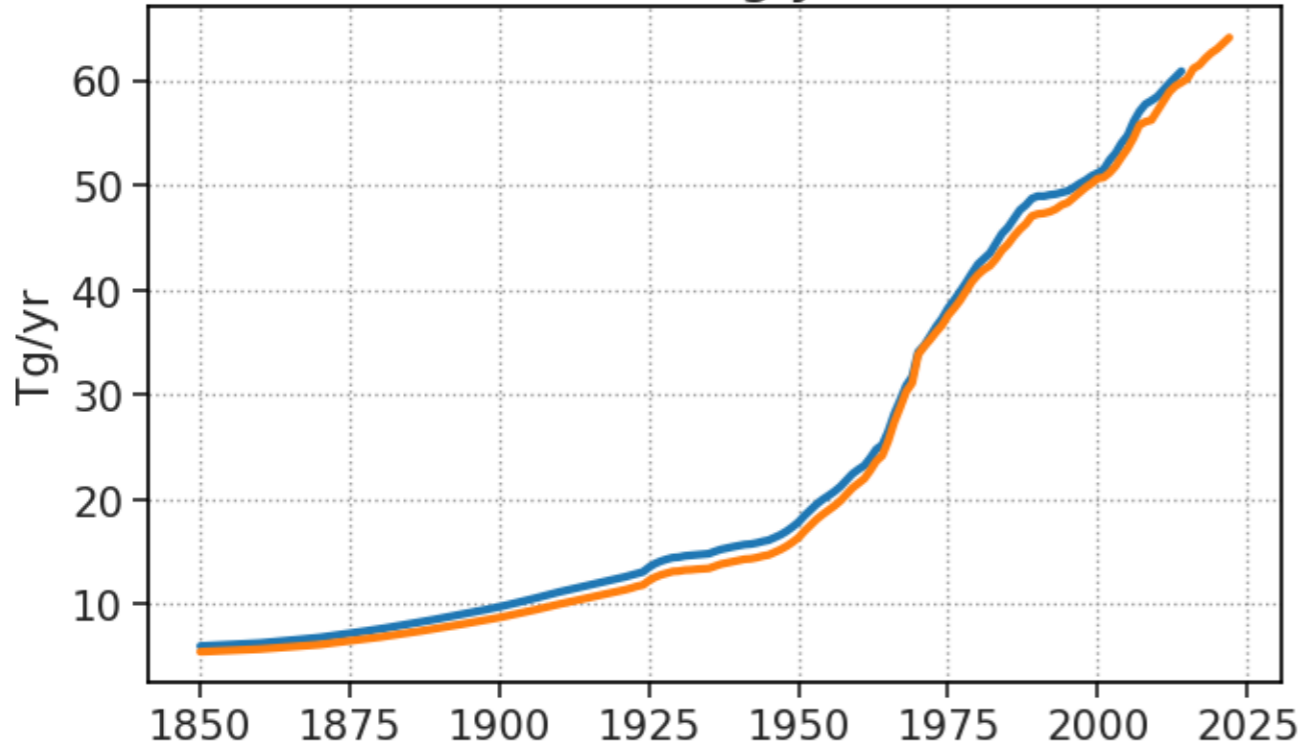
OC Tg/yr
