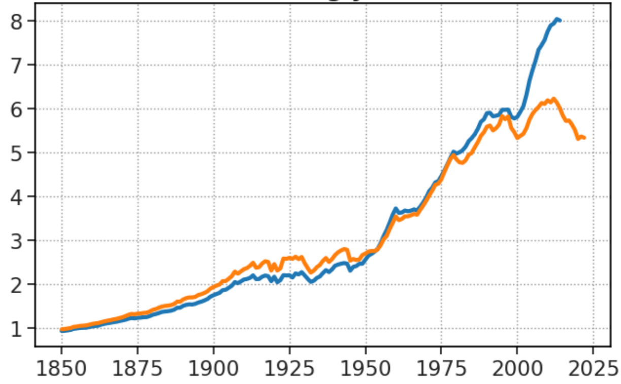
CO Tg/yr
