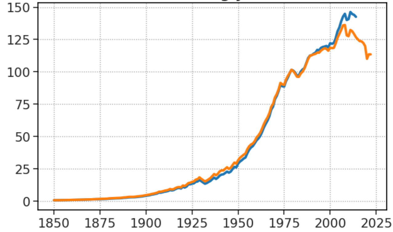
BC Tg/yr
